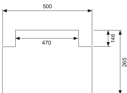
Rebate dimensions
