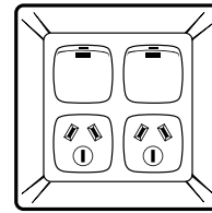
Twin Switched Socket with Neons 250V 10A P2025/2N #
