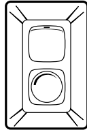
Single Light Dimmer and Switch to suit low voltage lights with iron-core transformers and incandescent lighting 220/250V 450W P2032E450L #
