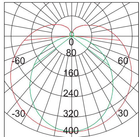
PHOTOMETRIC DIAGRAM
