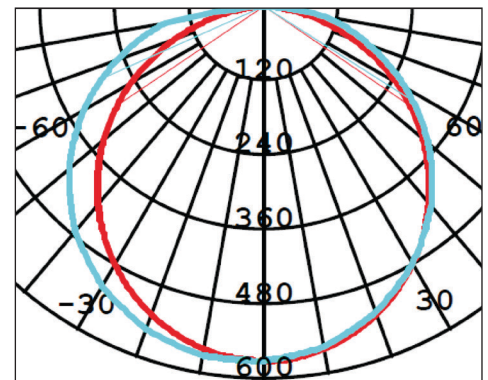
PHOTOMETRIC DIAGRAM
