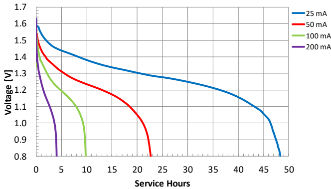
Constant Current
