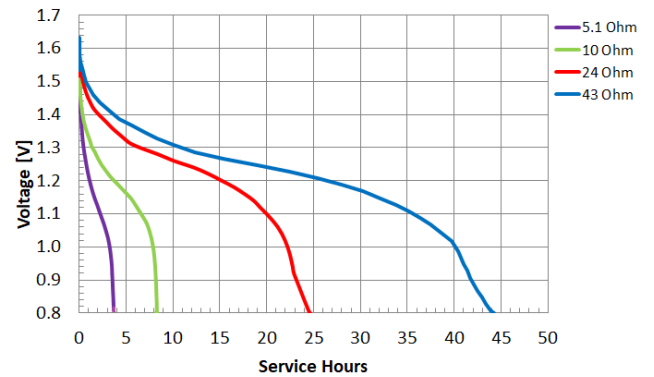
Constant Resistance
