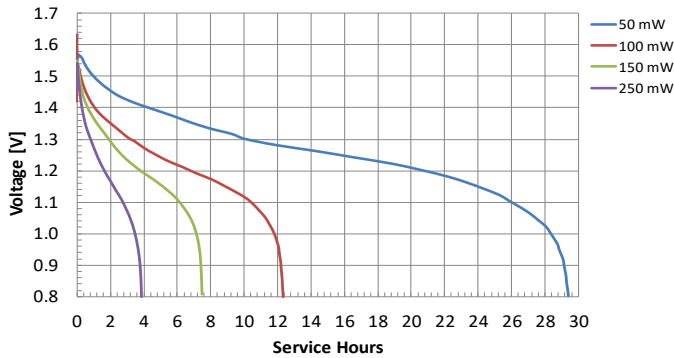
Constant Power
