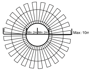
Height of Installation 2.5m Detection range
