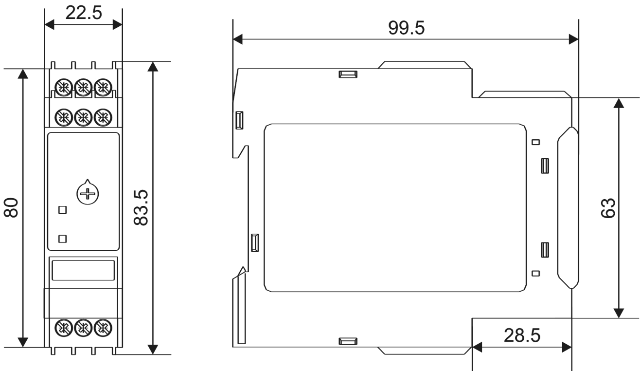
Dimension Diagram
