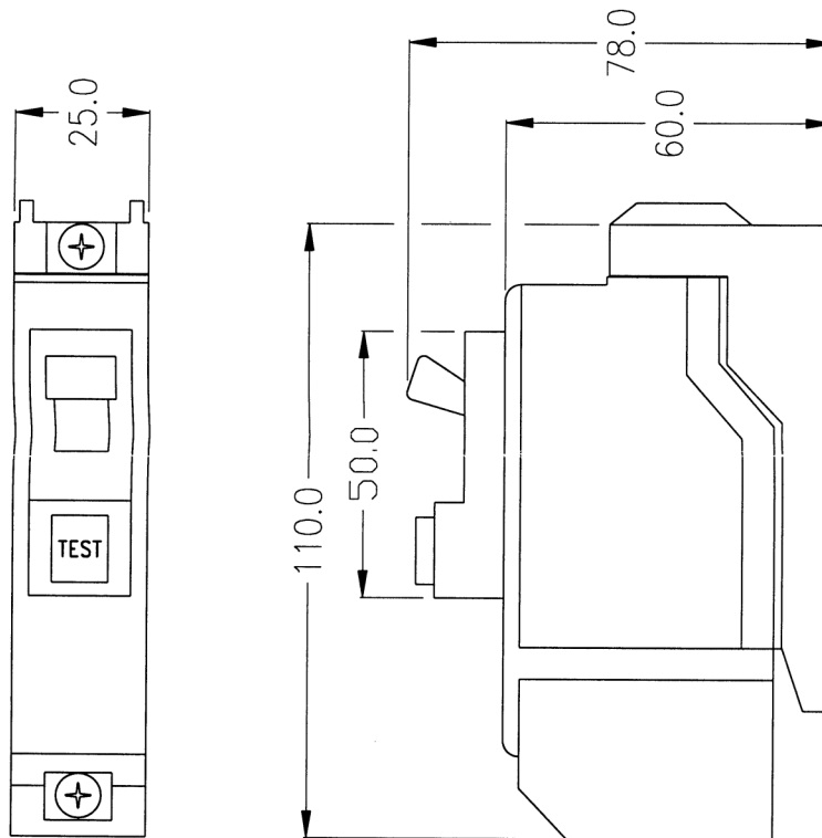
Dimension Diagram
