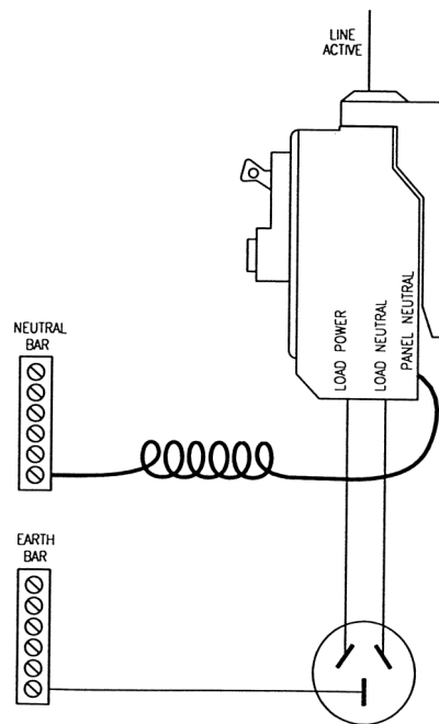
Connection / Wiring Diagram
