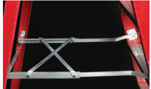
Cross Brace Locking System
