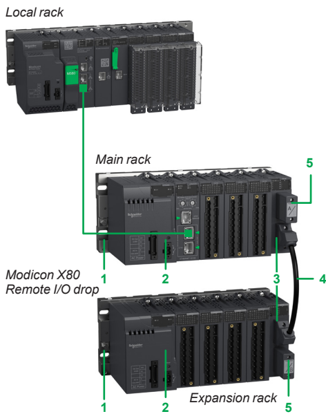
Modicon M580 local rack + Modicon X80 remote drop + expansion rack
