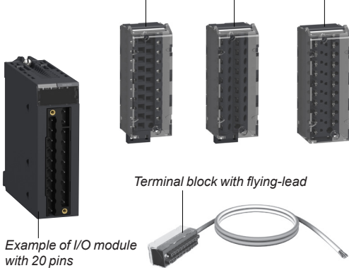
Accessories for connecting 20-pin modules
